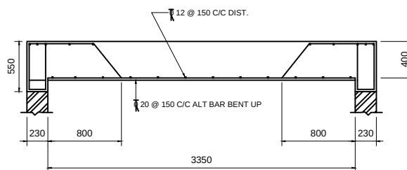
SECTION 1-1
